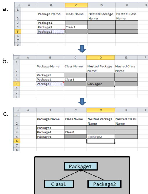
Figure 2.16: Defining Package2
